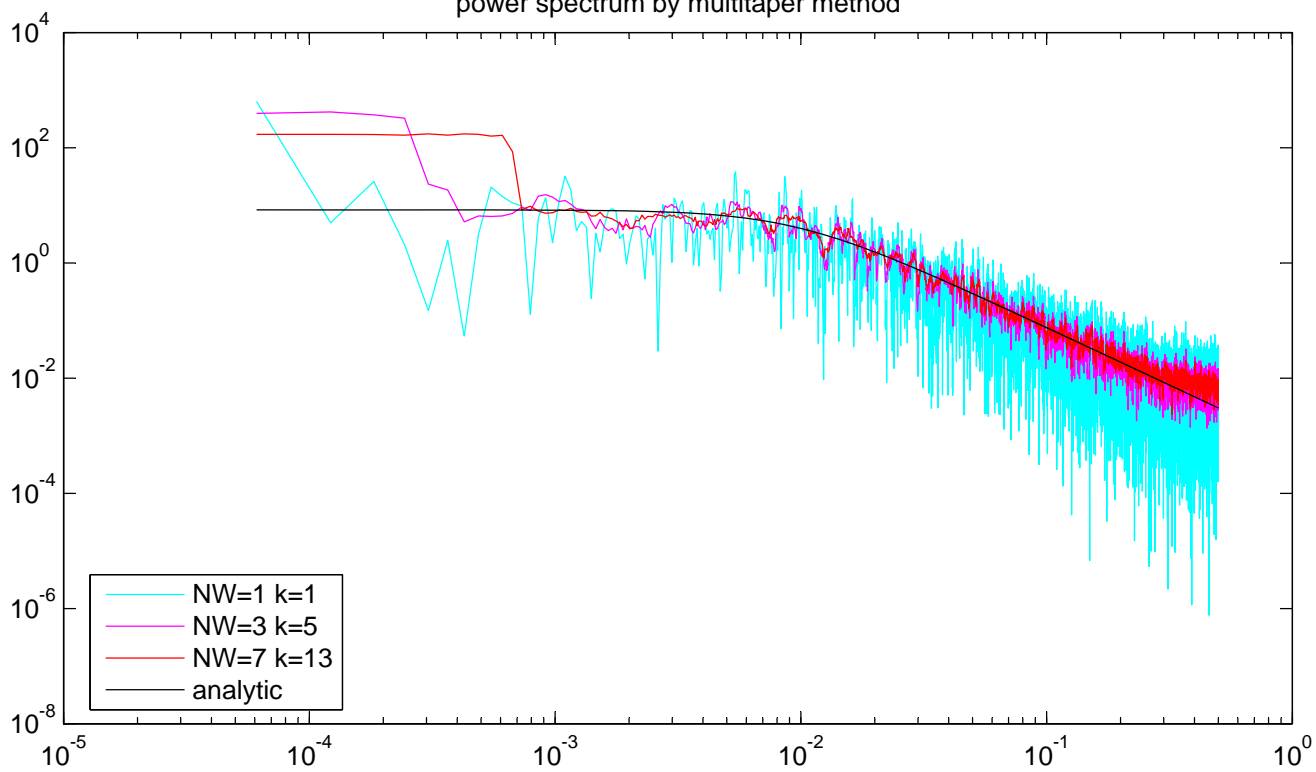
power spectrum by multitaper method
