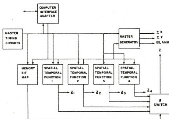
Figure 3. Block diagram of the instrument. The instrument comprises four spatial-temporal functions, a memory bit map, a fast analog Z switch, a raster generator, master timing circuits, and a computer interface adapter. The adapter distributes the computer-generated parameters to the instrument. Master timing circuits synchronize the generation of the raster with the intensity modulation produced on it. The raster generator provides a 256-line rotatable raster. The memory bit map assigns one of four spatial-temporal functions to each of 65,536 pixels in the raster by controlling the Z switch that selects the appropriate spatial-temporal function.
