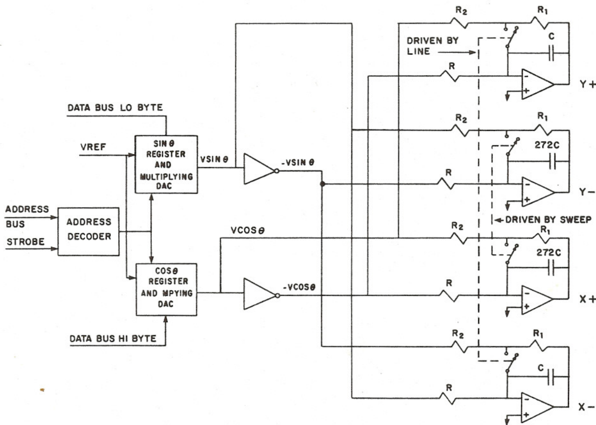
Figure 5. Raster generator. A 256-line rotatable raster is produced by the raster generator. The \sin and \cos of the rotation angle are provided by the computer. Voltages proportional to \pm\sin\theta and \pm\cos\theta are produced by the multiplying D/A converters and amplifiers. When the switches are open, linear ramps are produced by the four operational amplifiers. When the switches are closed, the ramps are reset to minus the value obtained at the end of the ramp. Thus rotation is provided around the center of the raster.
