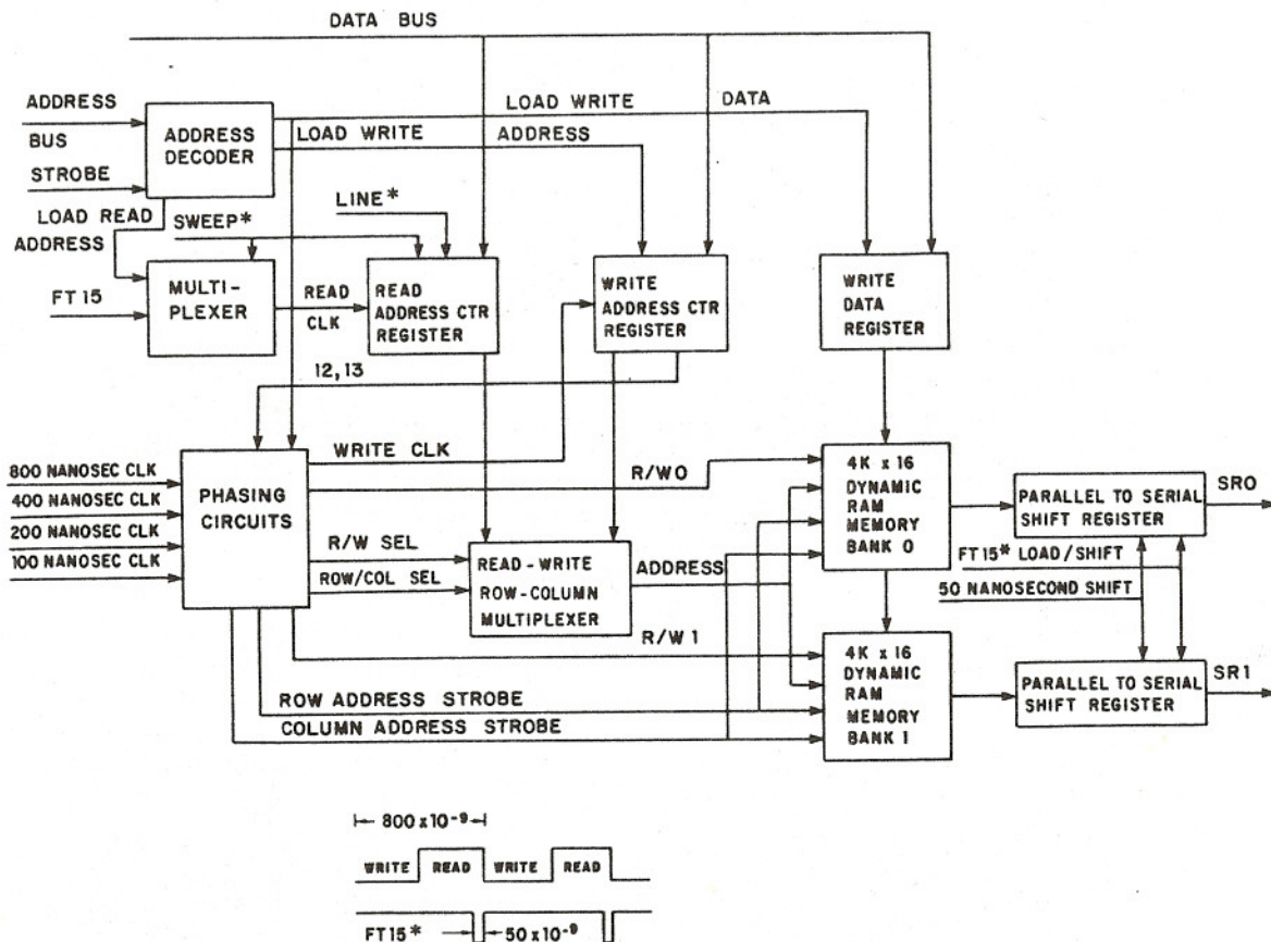
Figure 6. Memory bit map. The computer provides a 2-bit code for each of 65,536 pixels by filling up two 4,096 word by 16 bit dynamic memories. The locations are determined by the write address register, and their contents are provided by the data from the write data register. Each frame, 4,096 pairs of 16-bit words are read out of the RAMs from like locations in each memory bank into a pair of 16-bit parallel-to-serial shift registers. The addresses of the locations read are provided by the read address register. In each frame, the CRT beam traverses all the pixels. As the beam moves from one pixel to the next, a unique 2-bit code provided by the shift registers selects one of four possible independent spatial-temporal functions to modulate the beam.
