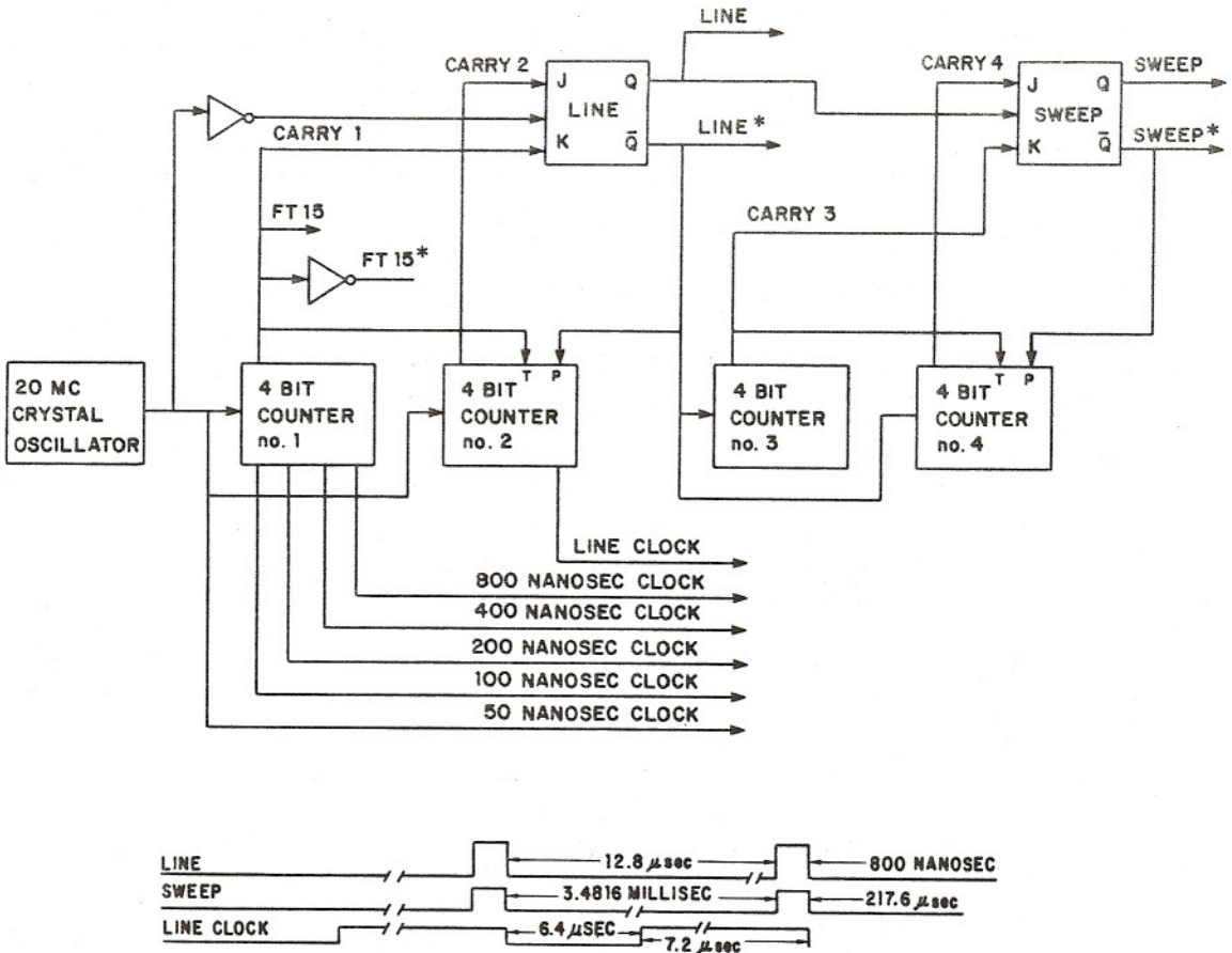
Figure 4. Master timing block diagram. The master timing circuits provide the timing signals required for synchronizing the raster generator with the modulation produced on it. The clocked signals are derived from a 20-MHz crystal oscillator driving two scale-of-272 cascaded counters.
