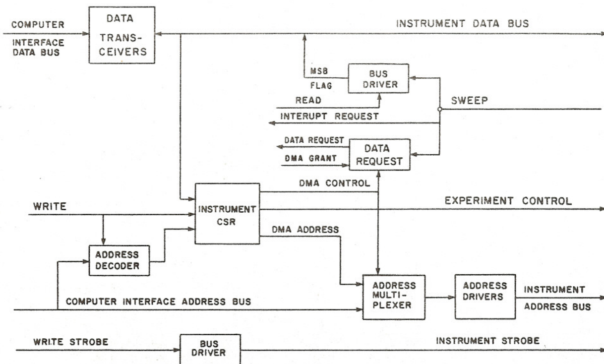
Figure 9. Computer interface adapter. Communication with the computer is accomplished through the interface adapter. The adapter receives information from the computer interface on 16-bit bidirectional data lines, three unidirectional address lines, and some control lines. Communication with the instrument is done over 16 bidirectional data lines, three address lines, one strobe line, and two control lines. The instrument CSR controls the mode of operation. During DMA transfers, the instrument address lines are provided by the CSR. Handshake logic controls the DMA transfers. During non-DMA transfers, the instrument address is supplied by the address lines from the computer interface. The address lines together with the strobe determines which function in the instrument is to receive the data on the data bus. The end-of-sweep signal is available to be used in an interrupt or flag mode to key the computer to update parameters.
