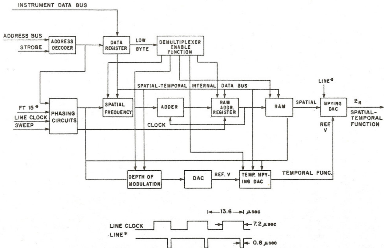
Figure 8. Spatial-temporal function. The computer supplies the intensity profile that resides in the RAM, the spatial frequency, the initial spatial address at the start of a frame, the depth of modulation, and the temporal function. In a typical experiment, the RAM, spatial frequency, and depth of modulation are initialized prior to an experimental run. During the run, at the end of each frame, the temporal function and/or the initial spatial address is updated. The RAM address register is clocked at the line generation rate. Hence the spatial function is a line function. The spatial-temporal output results from the triple product of depth of modulation, temporal function, and spatial function.
