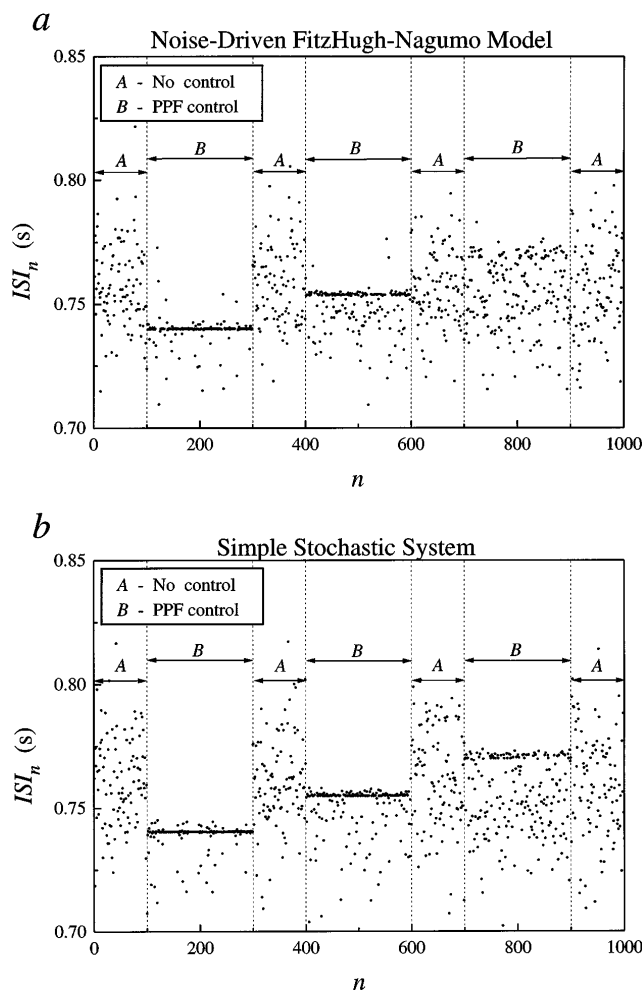
FIG. 3. (a) Plot showing interspike intervals ISI_n for the noise-driven, nonchaotic neuronal model without control (temporal regions A) and for three distinct periods of PPF control (regions B). For each PPF control region, a new apparent unstable periodic fixed point and set of apparent stable and unstable manifolds were determined during the preceding control-free region. (b) Plot showing three distinct periods of PPF control (regions B) of simulated interspike intervals ISI_n produced by the simple stochastic system [Eq. (2)].
