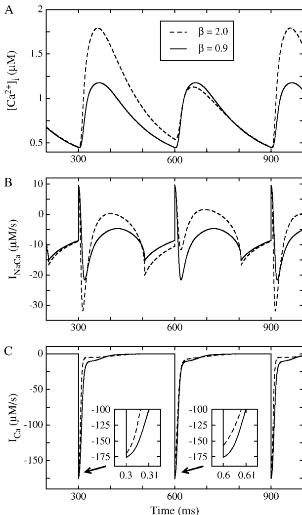
FIGURE 2 (A) Intracellular \text{Ca}^{2+} concentration, (B) \text{Na}^+ - \text{Ca}^{2+} exchange current, and (C) L-type \text{Ca}^{2+} channel current for two different values of \beta at a pacing period of T = 300 ms. When \beta = 2.0 , all three components exhibit a stable period-2 alternans rhythm. For \beta = 0.9 alternans does not occur in any component, indicating that the period-1, nonalternating rhythm is stable.
