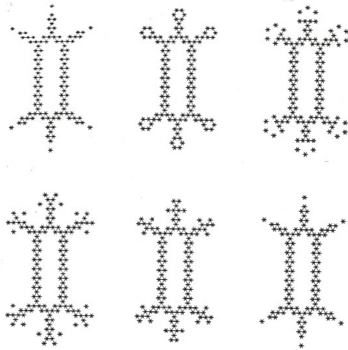
Fig. 3. An enclosure supported by rule (3422) (period 5).
