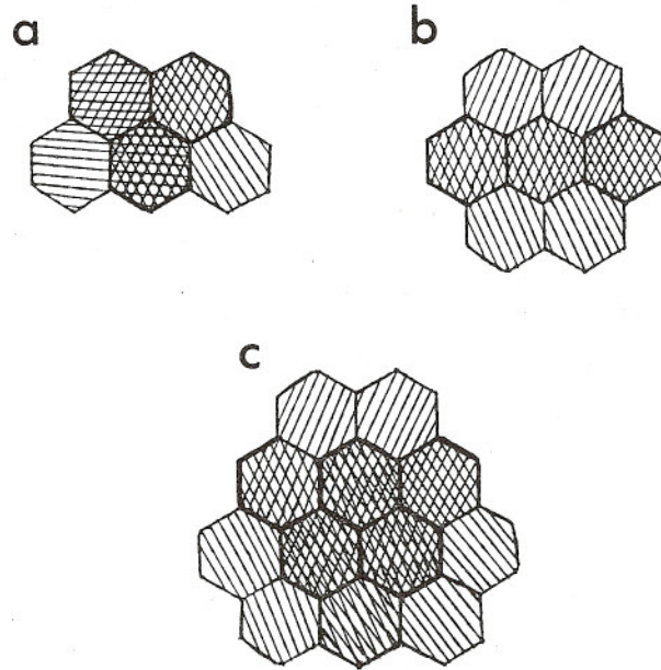
Fig. 7. (a) The extension of a block probability function on F_3 to a block probability function on F_5 . (b) The extension of a block probability function on F_5 to a block probability function on F_7 . (c) The extension of a block probability function on F_7 to a block probability function on F_{12} .
