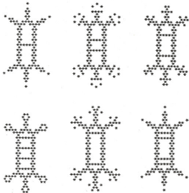
Fig. 4. An emulation within an enclosure by rule (3422) of the one-dimensional rule 90. Each successive picture represents two time-steps of rule (3422). This emulates one time-step of rule 90.
