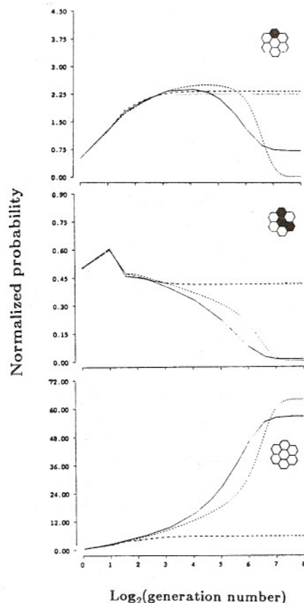
Fig. 9. Evolution of selected hexagon probabilities under (3422) on the hexagonal lattice. Monte-Carlo results (solid line) are compared to estimates from A_{F1} (dotted line), A_{F3} (dot-dash), and A_{F5} (dashed line). The normalized initial probability for each block is 0.5.
