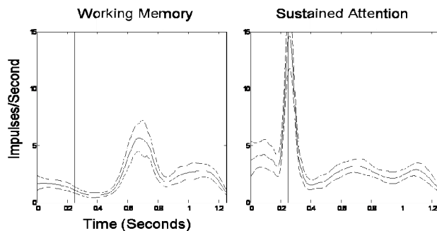
Fig. 1: A CT Single Unit firing rate response to a) Working memory; b) Sustained attention. The black vertical line represents the start of the delay period
